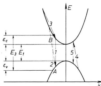
Fig. 1. Schematically E - k -diagram of the conduction band and the valence band to demonstrate different transition processes (arrows).
