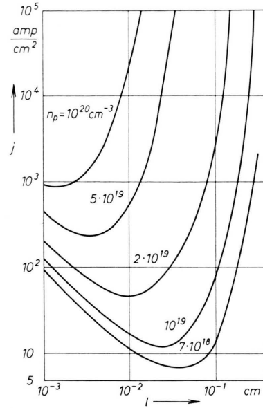
Fig. 3. Dependence of the lower bonds of current densities j to reach laser action, upon the slab length l and hole density n for a slab thickness d=0.37 \mu and end reflectivity R=99.5\% .
