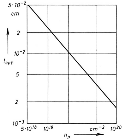
Fig. 4. Optimal slab length l_{\text{opt}} for smallest current densities as a function of hole density n_p .
