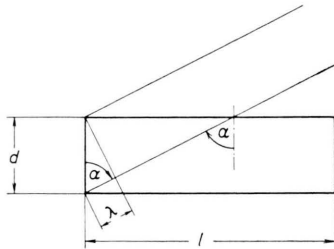
Fig. 2. To the discussion of diffraction losses.
